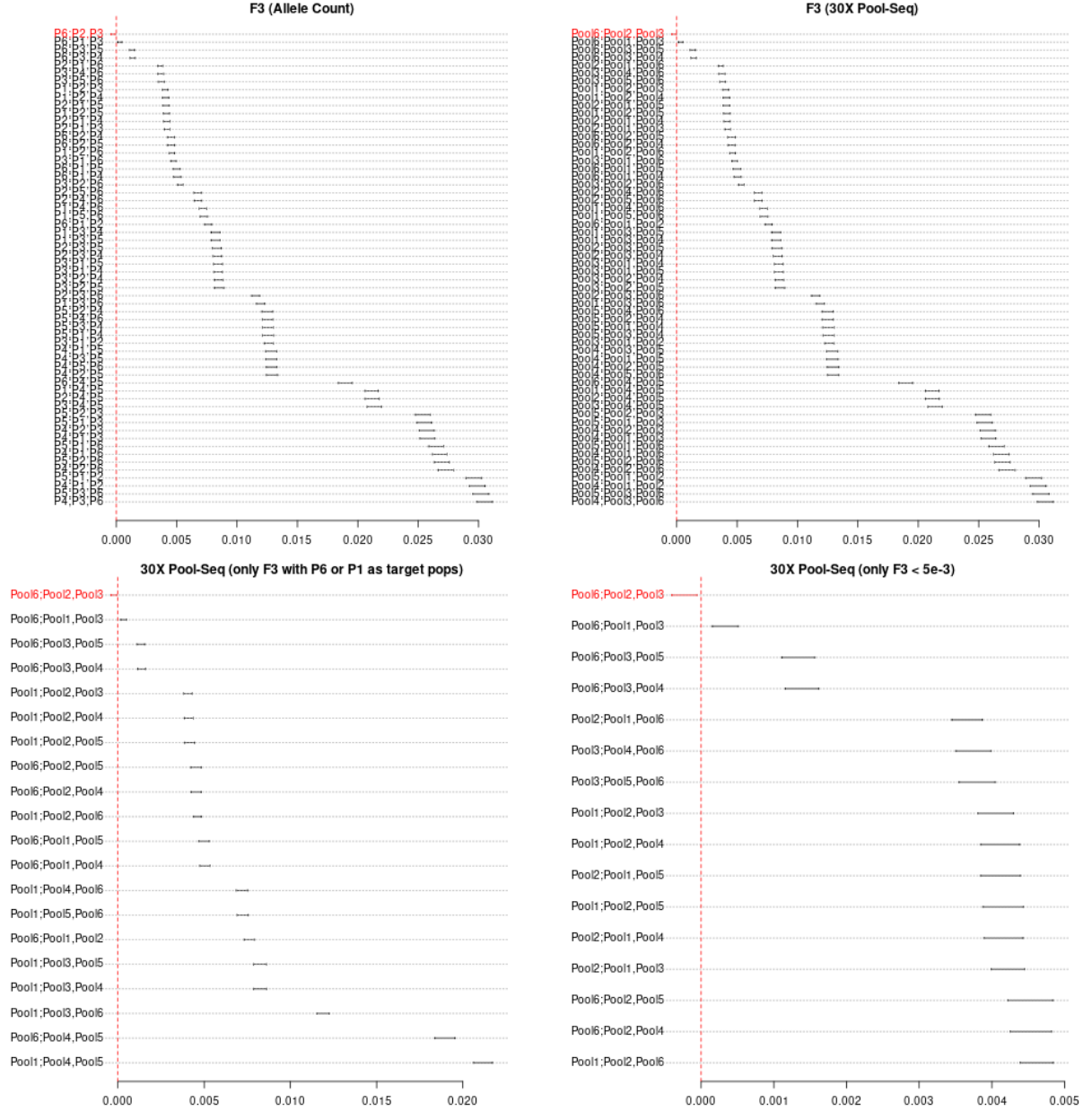
Figure 8: Estimated f_3 statistics with their 95% confidence intervals for the allele count and 30X Pool-Seq data sets
