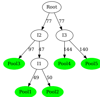
Figure 15: Plot of the rooted scaffold tree of unadmixed populations inferred by rooted.njtree.builder . The fitted edge lengths are in a drift scale (x1000).
