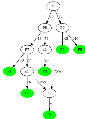
Figure 12: Plot of the admixture graph specifying the simulated scenario with fitted edge lengths scaled in drift units ( \times 1,000 )
