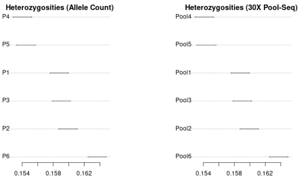
Figure 6: Estimated within-population heterozygosities with their 95% confidence intervals for the allele count and 30X Pool-Seq data sets
