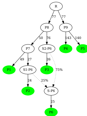
Figure 14: Plot of the graph with the lowest BIC among all the possible graphs connecting P6 to the five-population tree tested by the add.leaf . The fitted edge lengths are in drift units (x1000) since drift.scaling argument was set to TRUE when calling add.leaf .
