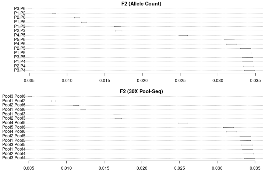
Figure 7: Estimated f_2 statistics with their 95% confidence intervals for the allele count and 30X Pool-Seq data sets
