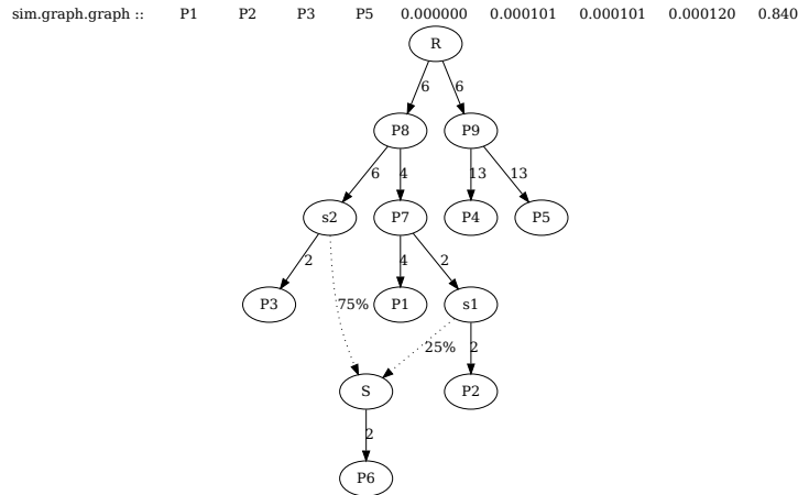
Figure 19: Fitting results obtained by qpGraph on the same data as the one used to generate Figure 11.
