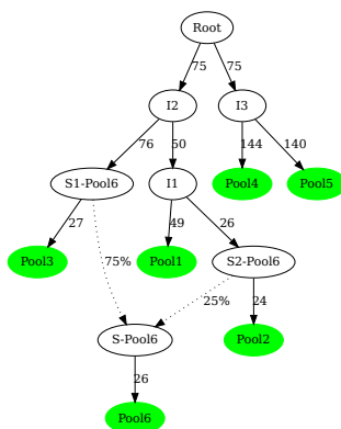
Figure 16: Plot of the graph with the lowest BIC among all the possible graphs connecting Pool6 to the scaffold tree of unadmixed population tested by the add.leaf . The fitted edge lengths are in drift units (x1000) since drift.scaling argument was set to TRUE when calling add.leaf .
